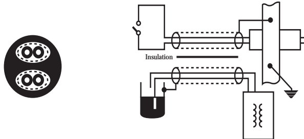
Figure 5: Limit switch and float switch in individually screened circuits bonded at different points
