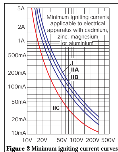
Figure 2 Minimum igniting current curves
